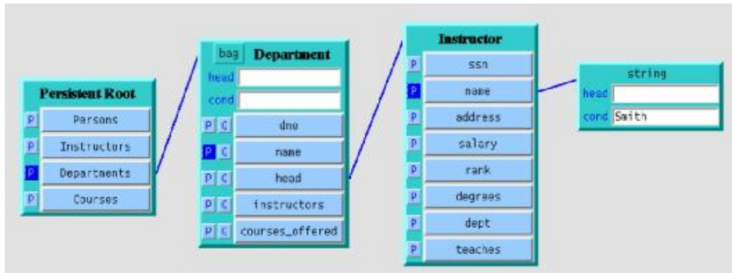
Figure 2. VOODOO query selecting the name of the department whose head is Smith.
