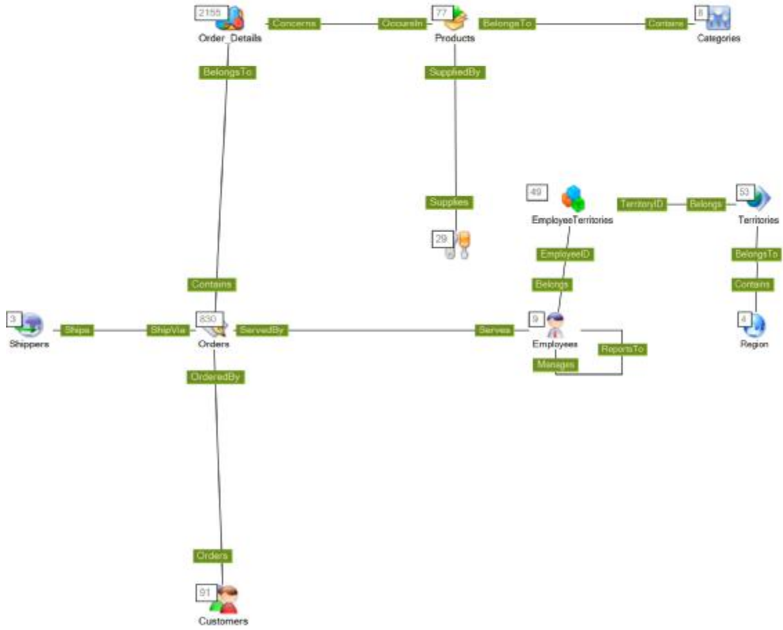
Figure 17. Intensional navigation graph
