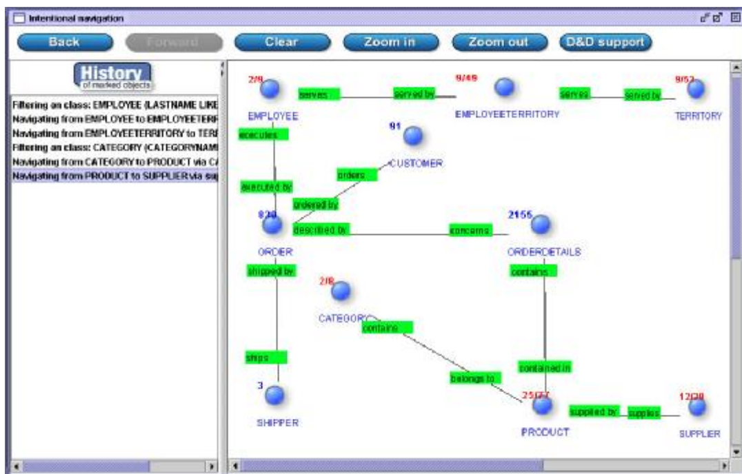
Figure 26. Structural Knowledge Graph Navigator (SKGN) during intensional navigation
