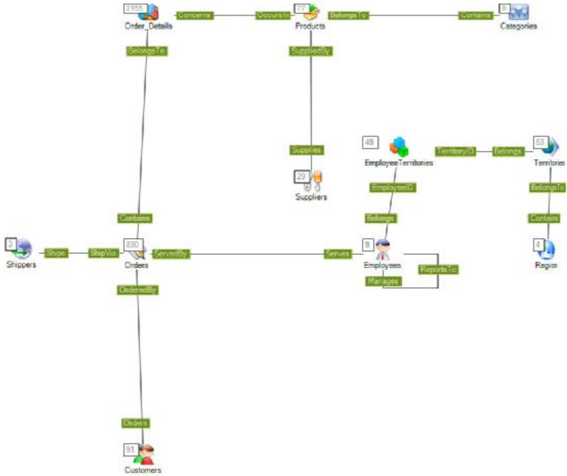
Figure 24. Example of a database virtual schema
