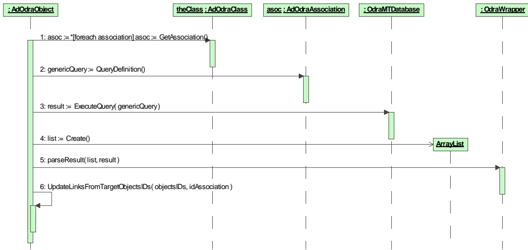
Figure 75. Sequence diagram for creating an object – part (b).
