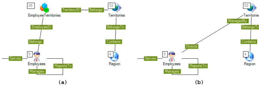
Figure 25. Illustration of hiding intermediary classes.
